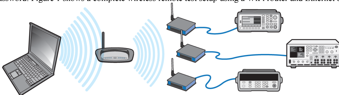
Figure 1. Wireless test setup using a WiFi router and Ethernet bridges
